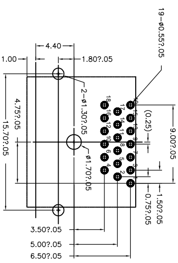
RECOMMENDED PCB LAYOUT(T=1.60±0.15) COMPONENT SIDE
